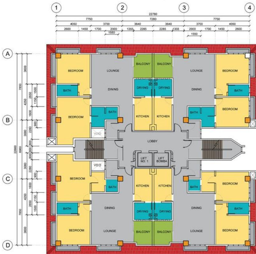
TYPICAL 1ST - 6TH FLOOR PLAN Scale 1:100
